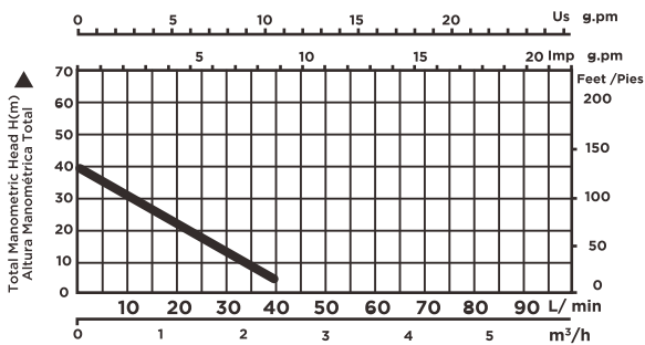
PERFORMANCE CURVE - CURVA DE EFICIENCIA N=3,450 R/MIN
