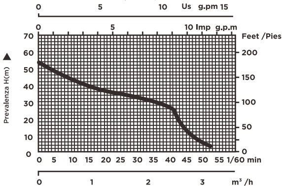
PERFORMANCE CURVE - CURVA DE EFICIENCIA N=3,450 R/MIN
