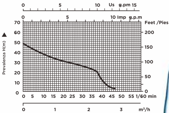
PERFORMANCE CURVE - CURVA DE EFICIENCIA N=3,450 R/MIN - PS12235
