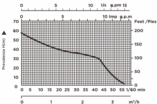
PERFORMANCE CURVE - CURVA DE EFICIENCIA N=3,450 R/MIN - PS12238
