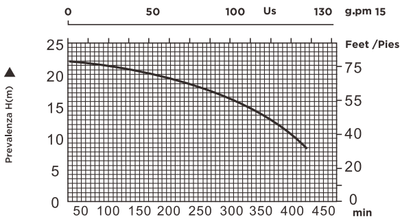
PERFORMANCE CURVE - CURVA DE EFICIENCIA N=3,450 R/MIN
