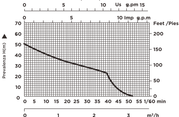
PERFORMANCE CURVE - CURVA DE EFICIENCIA N=3,450 R/MIN
