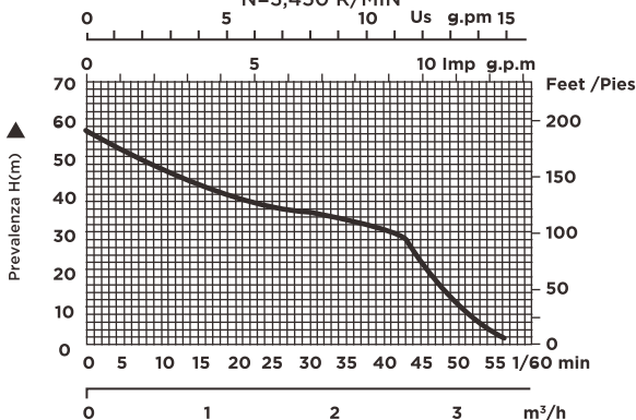
PERFORMANCE CURVE - CURVA DE EFICIENCIA N=3,450 R/MIN
